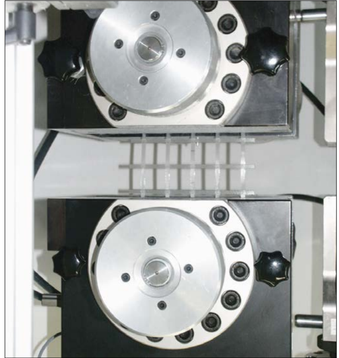
Fig. 12 Tensile strength testing of Secugrid®
