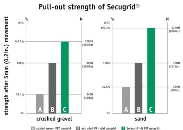
Fig. 15 Soil pull-out results with 3 geogrids
