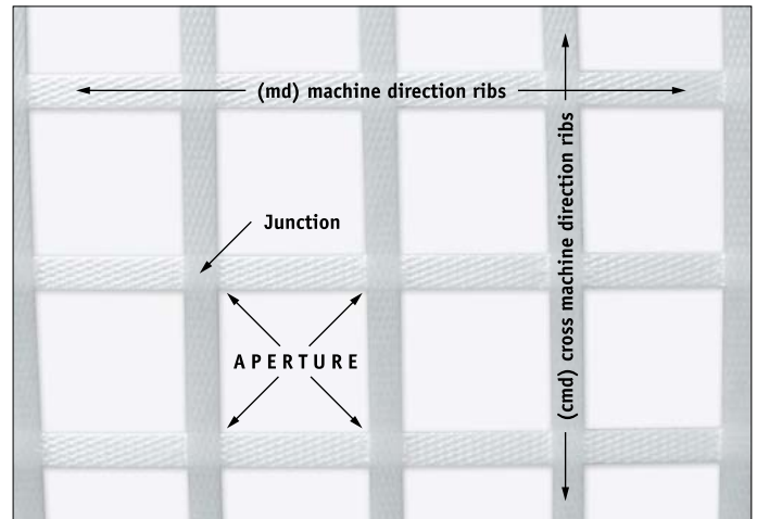
Fig. 1 Geogrid definitions
