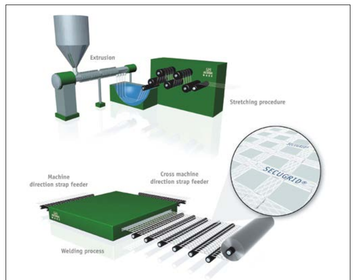
Fig. 5 Secugrid® manufacturing process
