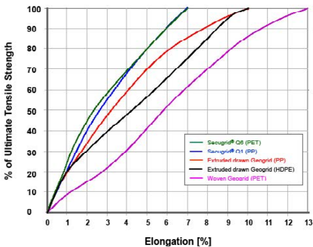
Fig. 13 Stress-strain curves of Secugrid® and selected geogrids
