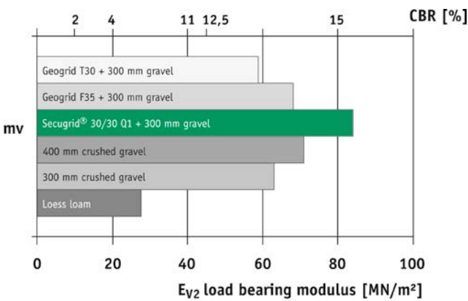
Fig. 18 Performance of Secugrid® compared to other geogrid reinforced sections as base course stabilisation
